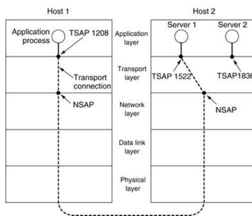
TSAPs, NSAPs and transport connections.
