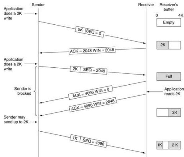
Window management in TCP.
