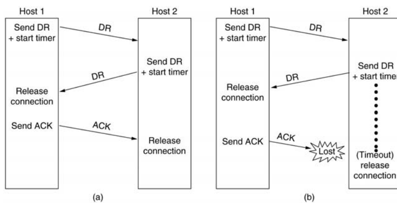
Four protocol scenarios for releasing a connection. (a) Normal case of a three-way handshake. (b) final ACK lost.
