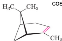
\alpha -Pinene
