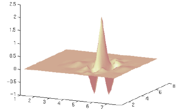
coif2: psi(x)*psi(y).
