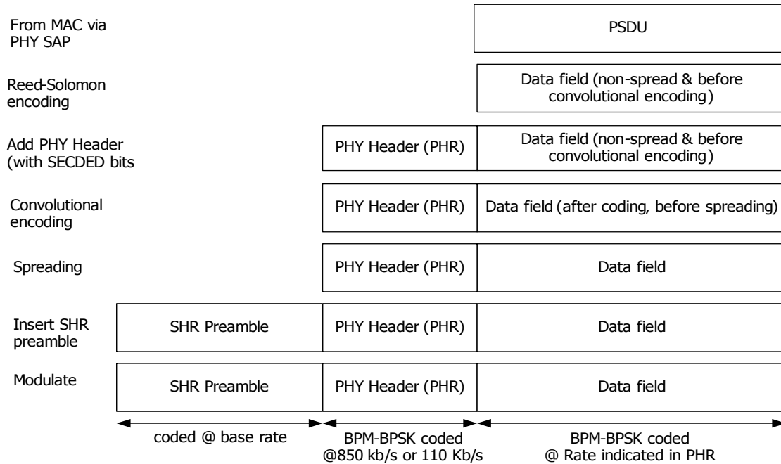
Figure 84—UWB PDU encoding process
