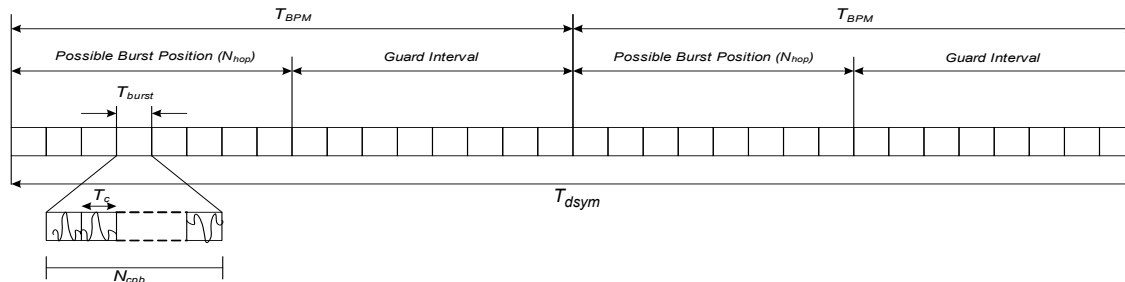
Figure 85—UWB PHY symbol structure
