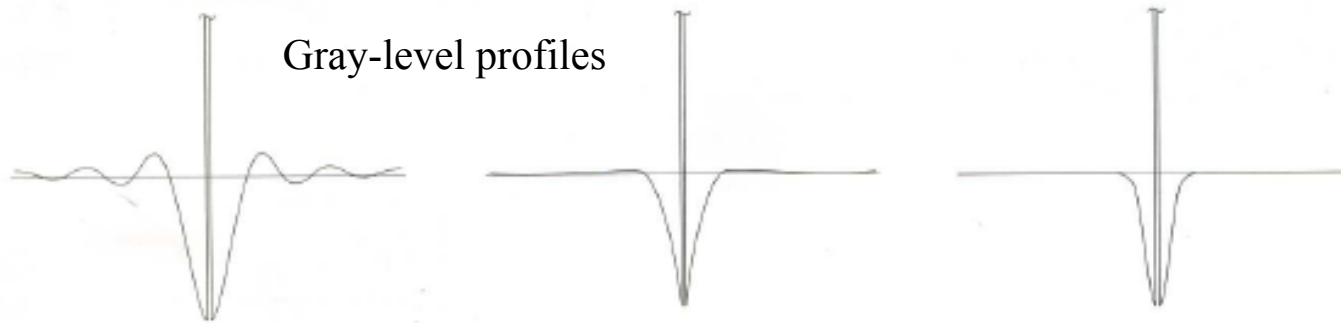
FIGURE 4.23 Spatial representations of typical (a) ideal, (b) Butterworth, and (c) Gaussian frequency domain highpass filters, and corresponding gray-level profiles.
