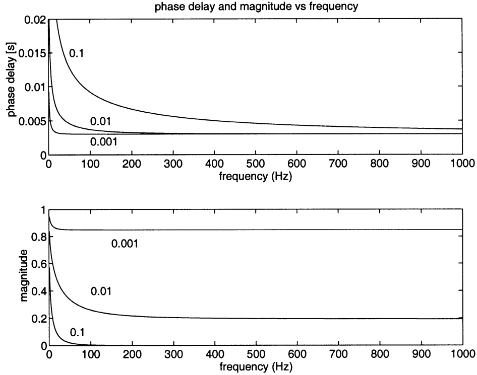
Fig. 4. Phase delay (in seconds) and magnitude response introduced by frictional losses in a waveguide section of length L_R = 1 , for different values of \Upsilon .
