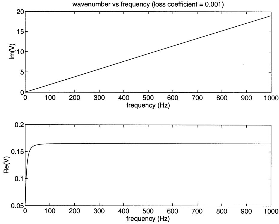
Fig. 2. Imaginary and real part of the wave number as functions of frequency ( \Upsilon = 0.001 ).
