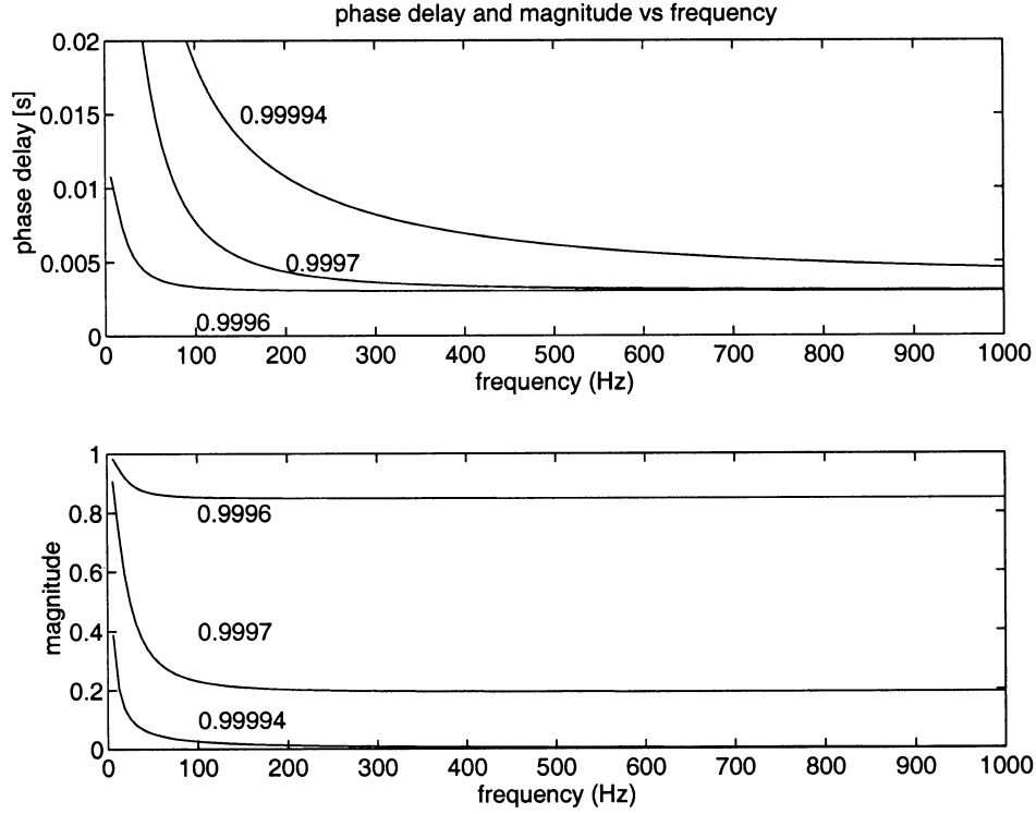
Fig. 5. Phase delay (in seconds) and magnitude response of a first-order IIR filter, for different values of the coefficient r , \alpha is set to 1 - e^{-(1/2)\Upsilon cL_R} with the same values of \Upsilon used for the curves in Fig. 4.
