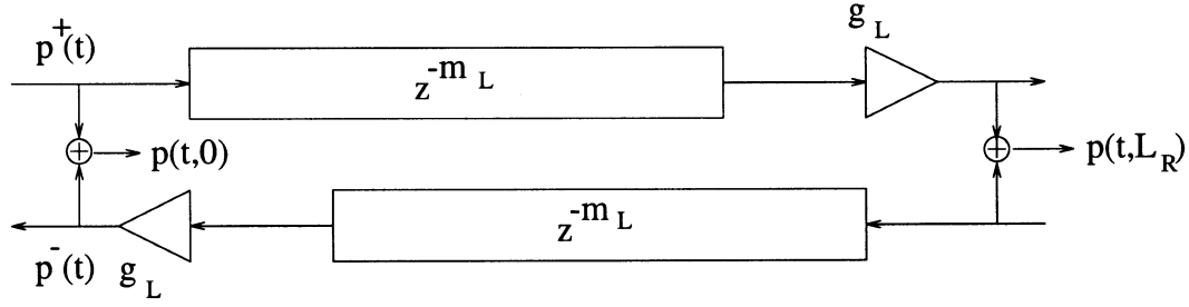
Fig. 3. Length- L_R one-variable waveguide section with small losses.
