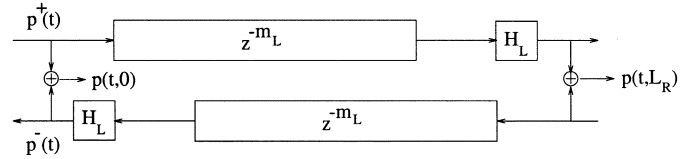
Fig. 6. Length- L_R one-variable waveguide section with small losses.
