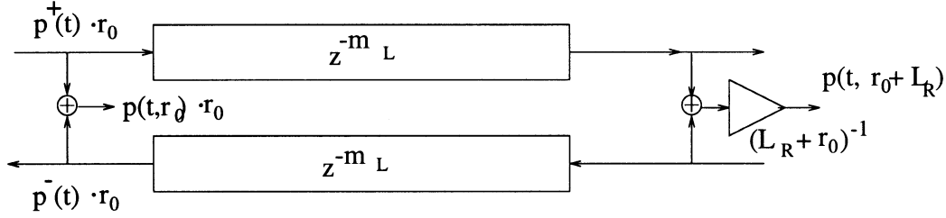
Fig. 8. One-variable waveguide section for a length- L_R conical tract.
