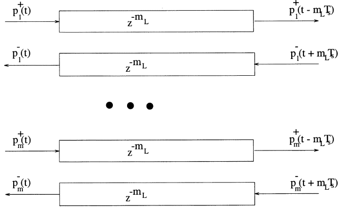
Fig. 1. An m -variable waveguide section.
