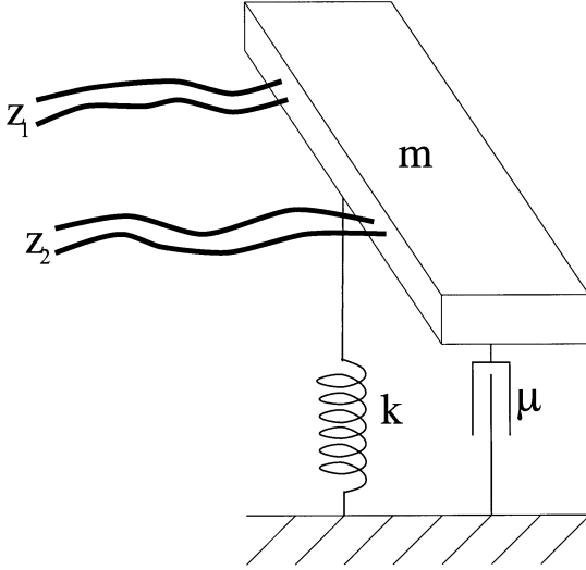
Fig. 7. Two pairs of strings coupled at a bridge.
